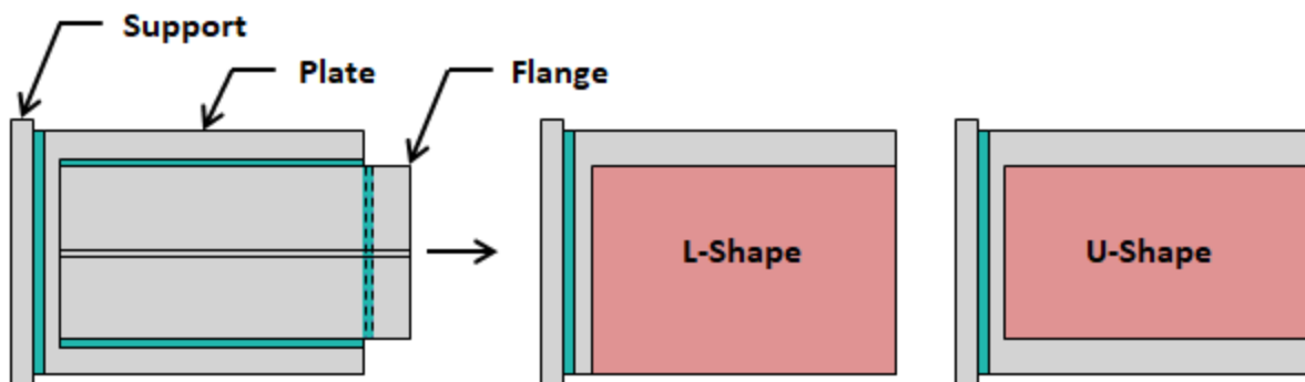
Block Shear Failure Modes – End Weld & Plate Width > Flange Width
