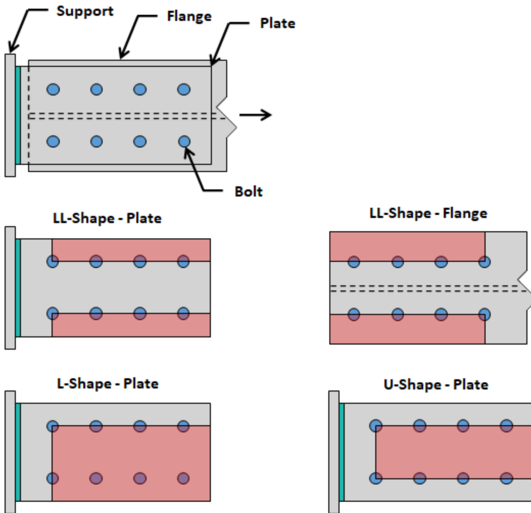
Block Shear Failure Modes
