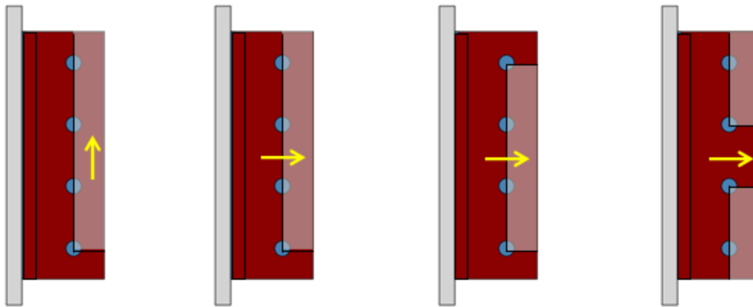
(a) Shear L-Shape (b) Tension L-Shape (c) Tension U-Shape (d) Tension LL-Shape
