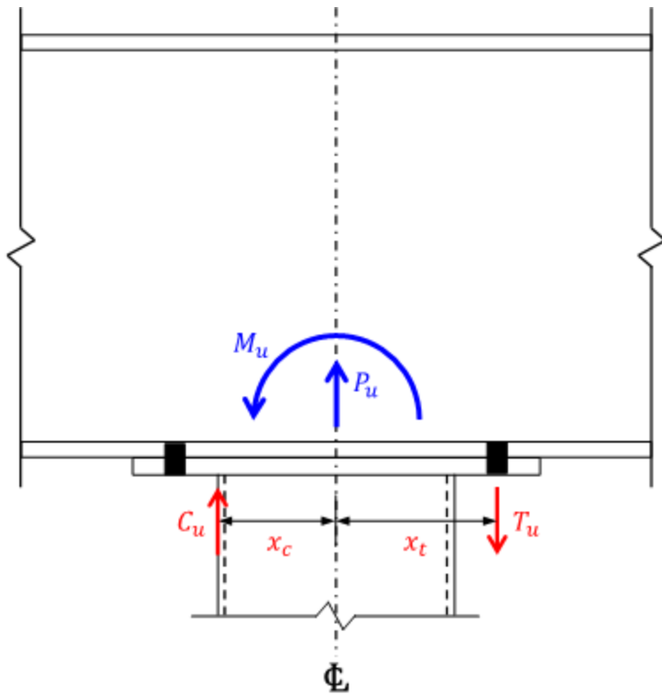
Beam Over HSS Connection Statics
