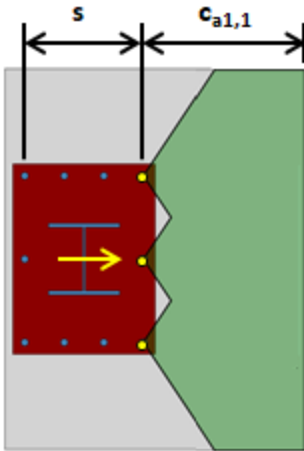
Concrete Breakout for Anchor Group – Case 3
