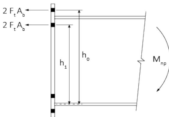
4 Bolt Configuration
